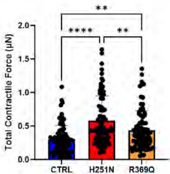
Figure 1: Traction Force Microscopy contractility analysis reveals genotype-induced hypercontractility by the H251N mutation
